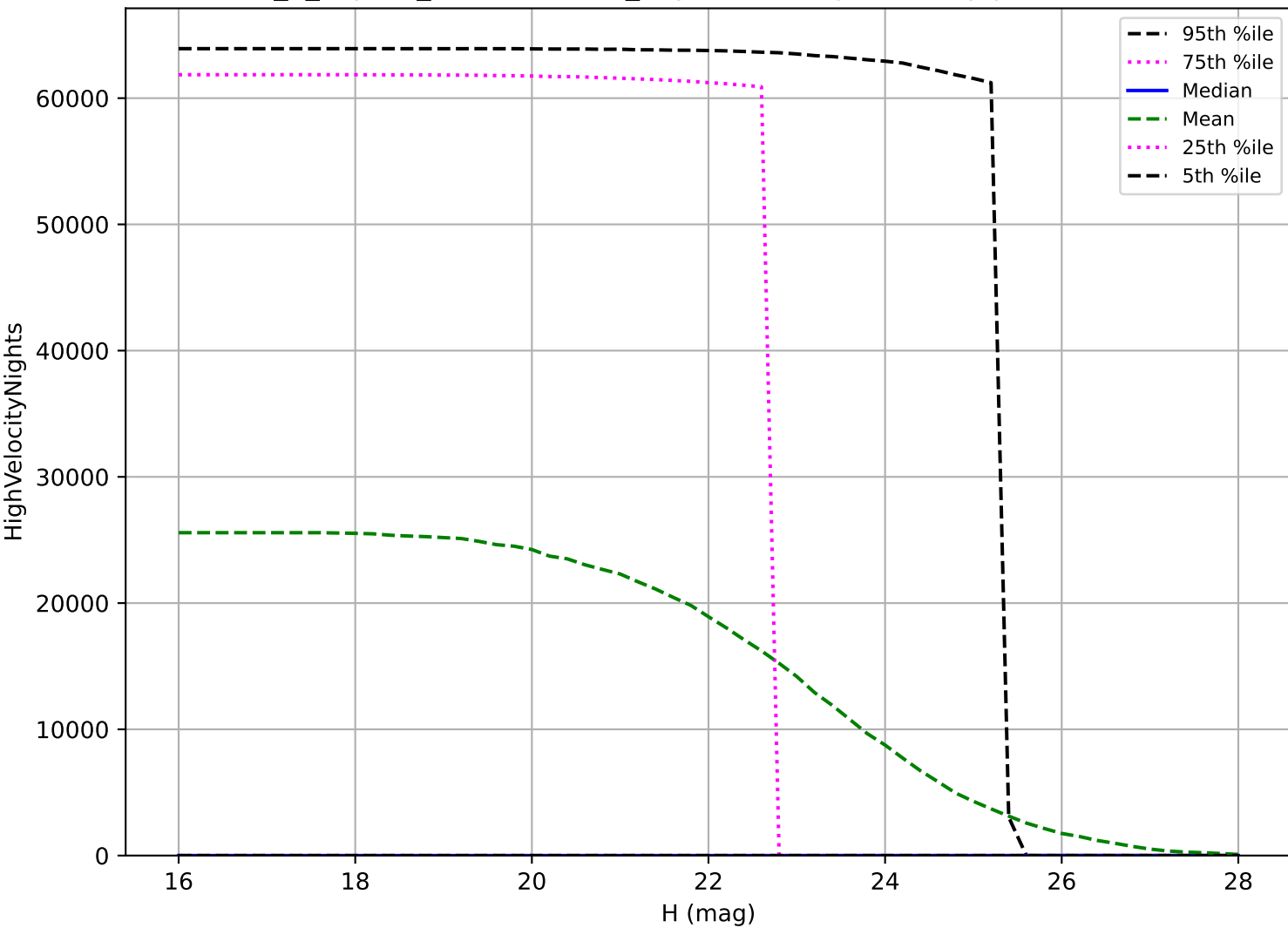
internal_u_expt60_nscale1.0v3.4_10yrs: PHA High velocity pair detection loss
