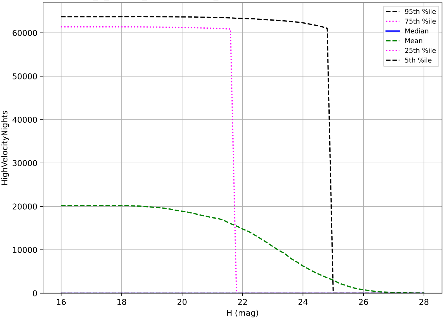
internal_u_expt60_nscale1.0v3.4_10yrs: NEO High velocity pair detection loss
