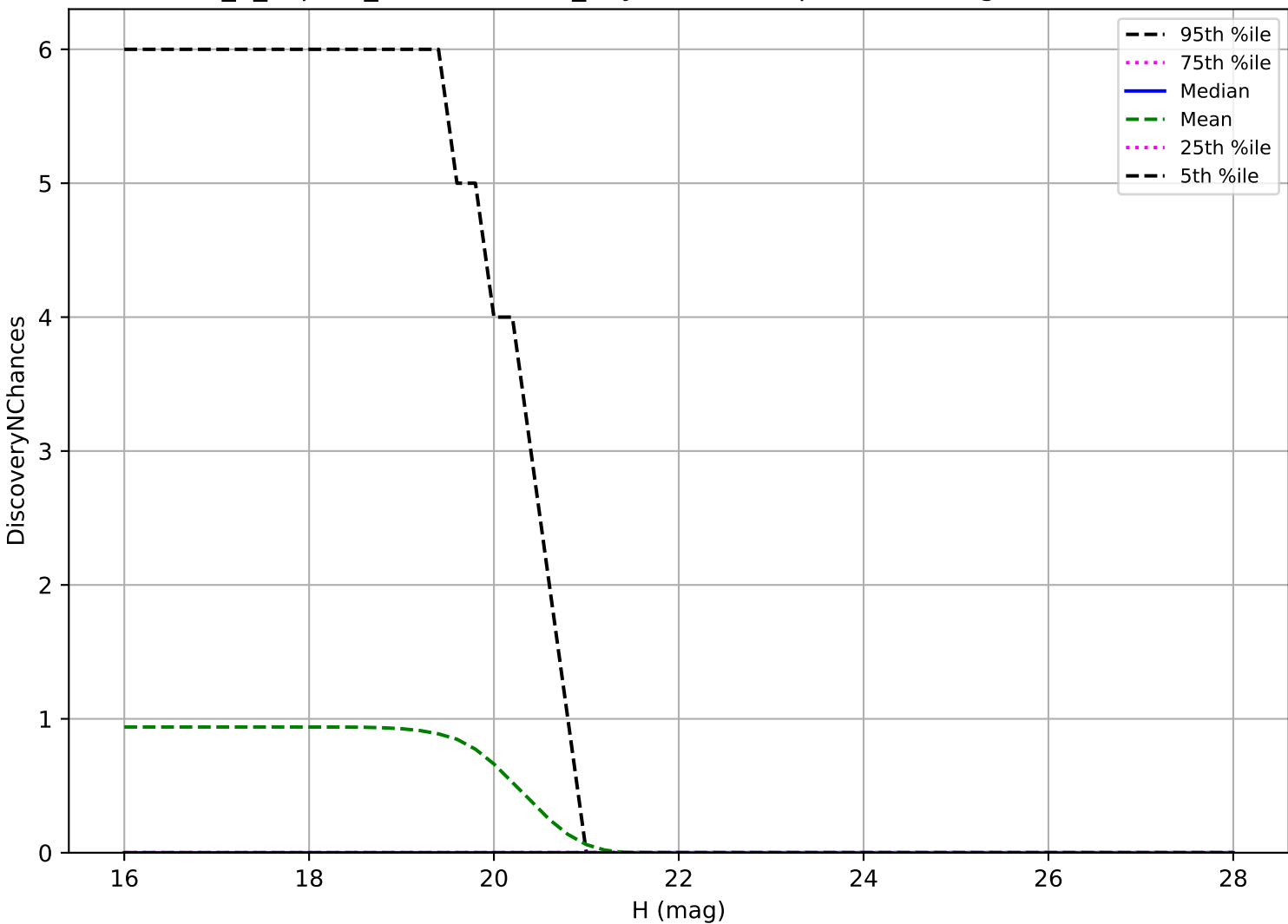
internal_u_expt60_nscale1.0v3.4_10yrs: Vatira 3 pairs in 15 nights detection loss
