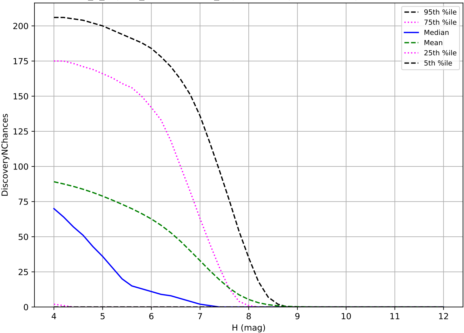
internal_u_expt60_nscale1.0v3.4_10yrs: TNO 3 pairs in 15 nights detection loss
