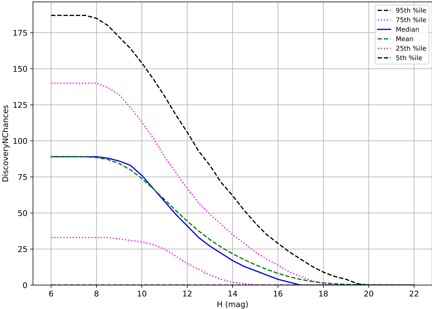
internal_u_expt60_nscale1.0v3.4_10yrs: OCC_r5 3 pairs in 15 nights detection loss
