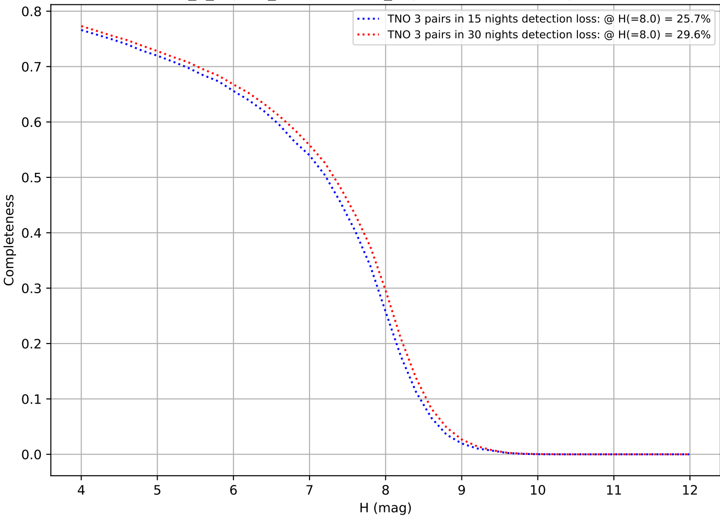
internal_u_expt60_nscale1.0v3.4_10yrs: DifferentialCompleteness
