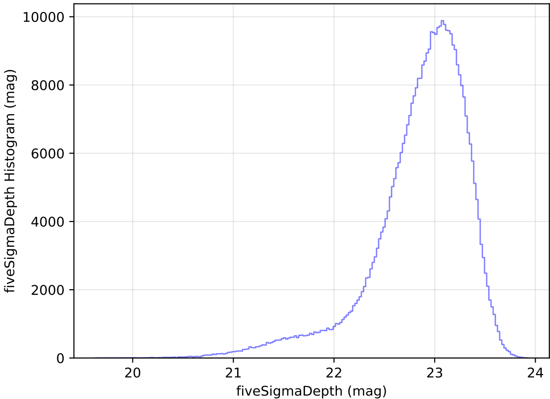
internal_u_expt60_nscale1.0v3.4_10yrs z: fiveSigmaDepth Histogram
