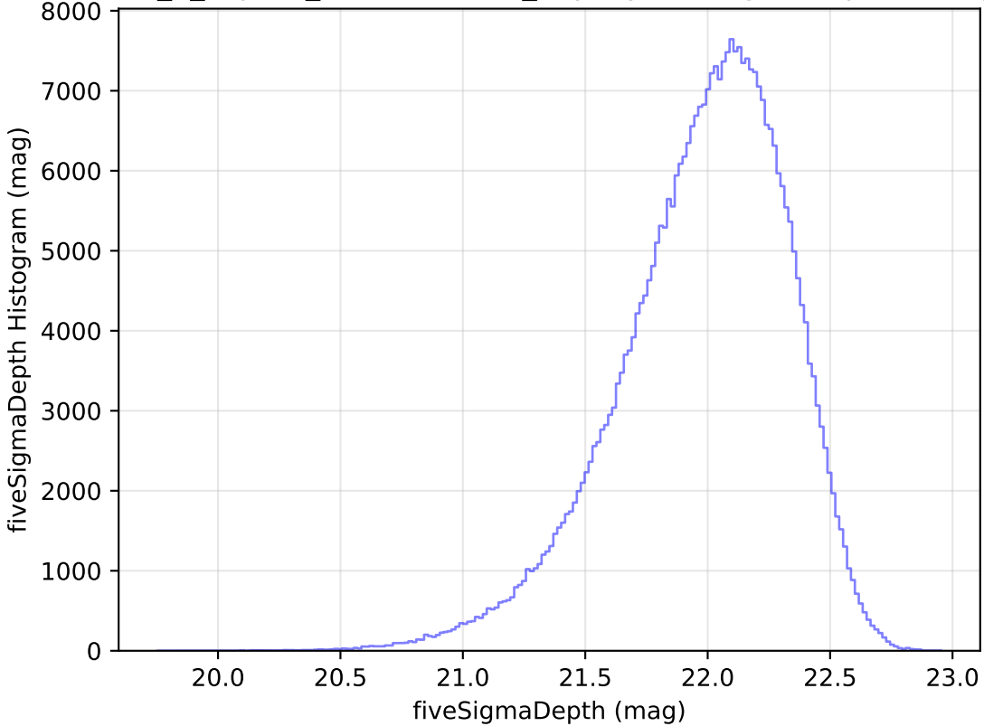
internal_u_expt60_nscale1.0v3.4_10yrs y: fiveSigmaDepth Histogram
