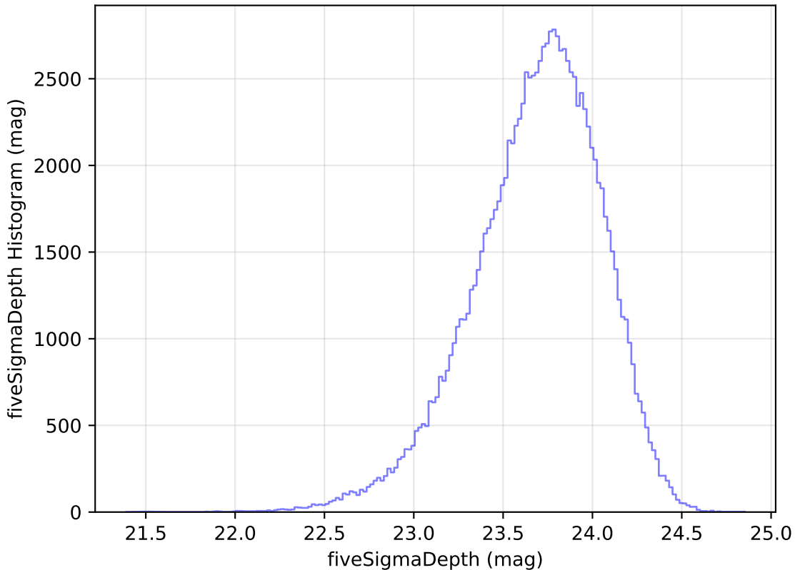
internal_u_expt60_nscale1.0v3.4_10yrs u: fiveSigmaDepth Histogram
