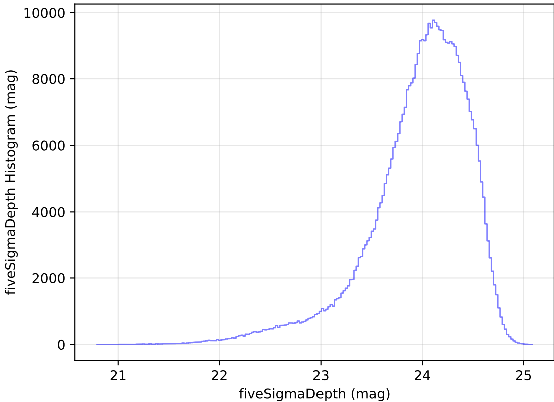
internal_u_expt60_nscale1.0v3.4_10yrs r: fiveSigmaDepth Histogram
