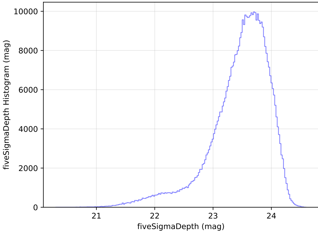
internal_u_expt60_nscale1.0v3.4_10yrs i: fiveSigmaDepth Histogram
