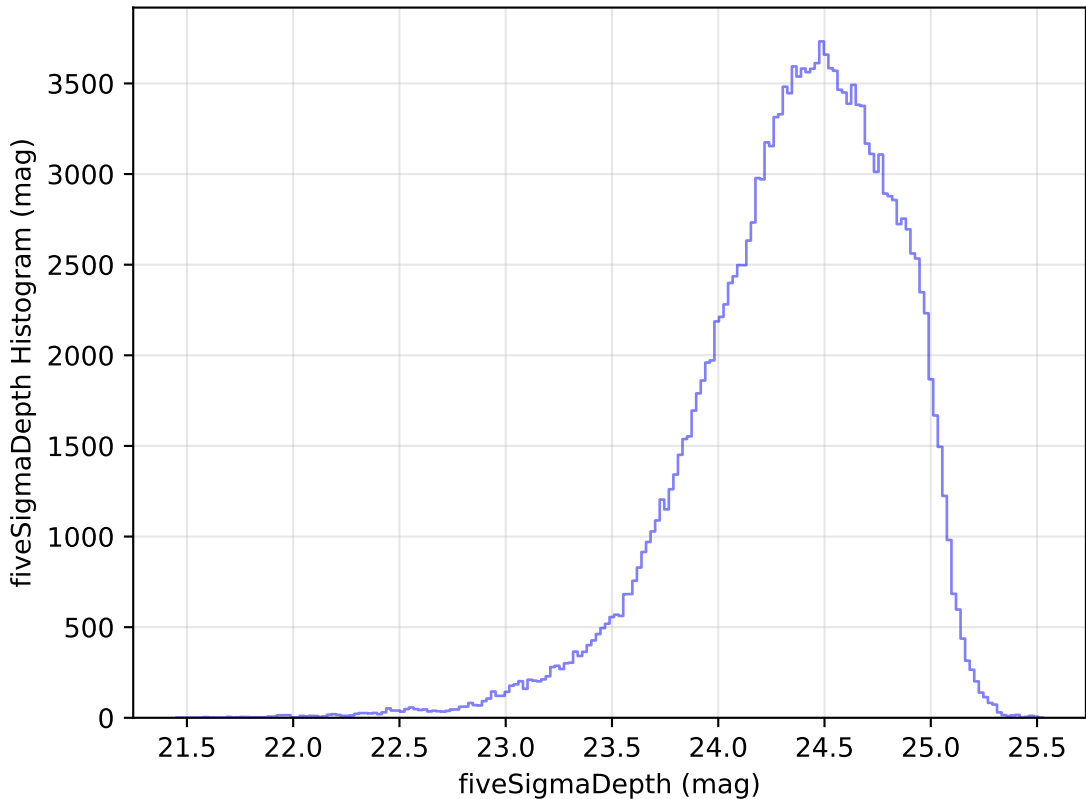
internal_u_expt60_nscale1.0v3.4_10yrs g: fiveSigmaDepth Histogram
