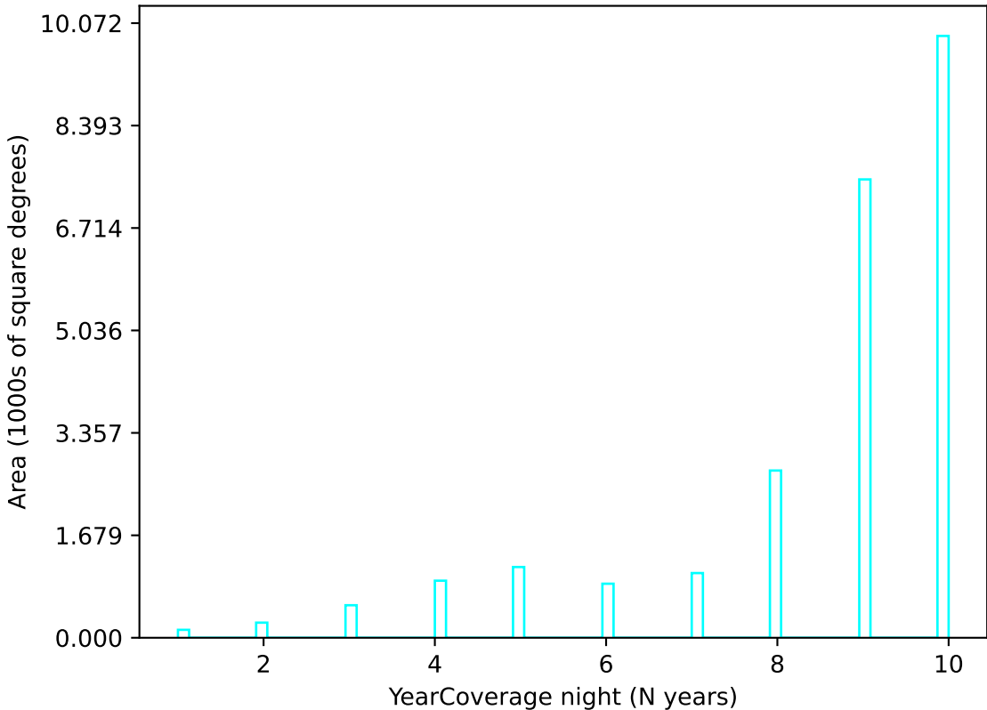
internal_u_expt60_nscale1.0v3.4_10yrs u band: YearCoverage night
