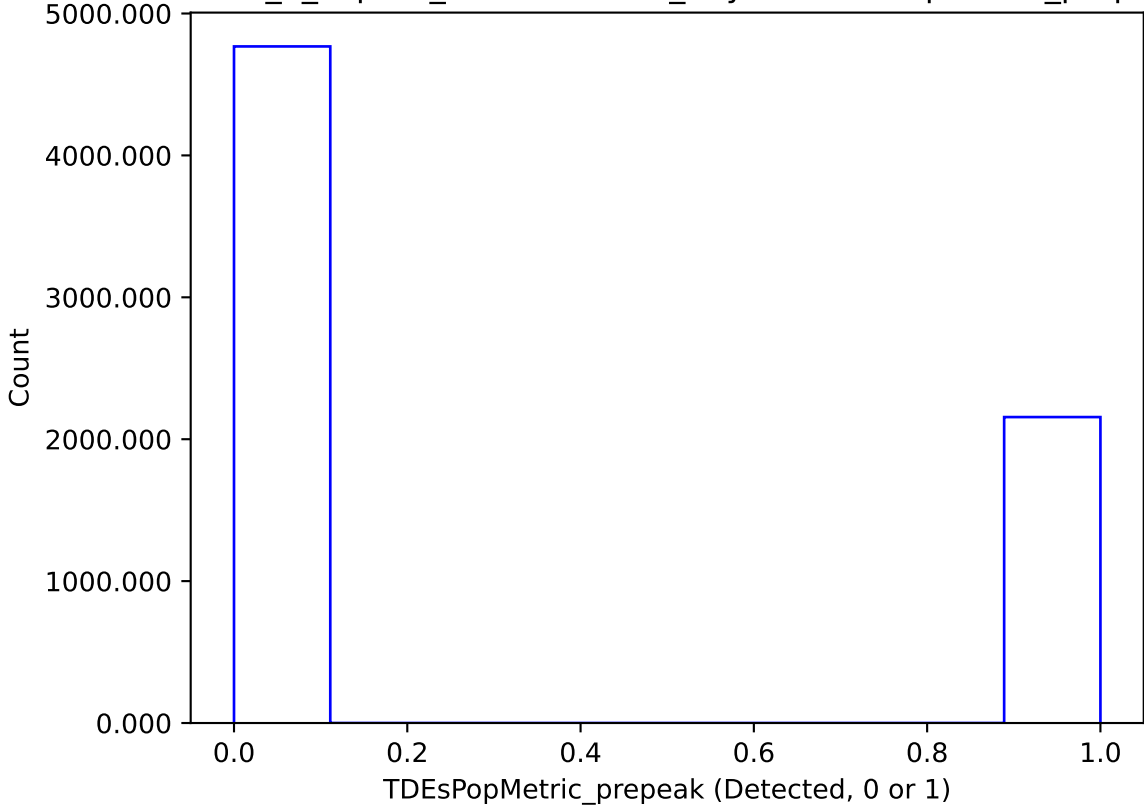
internal_u_expt60_nscale1.0v3.4_10yrs : TDEsPopMetric_prepeak
