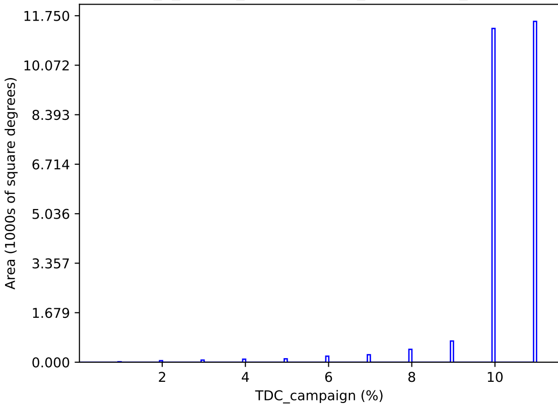
internal_u_expt60_nscale1.0v3.4_10yrs : TDC_campaign
