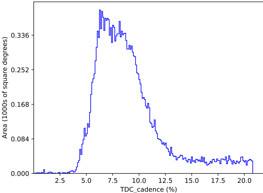
internal_u_expt60_nscale1.0v3.4_10yrs : TDC_cadence
