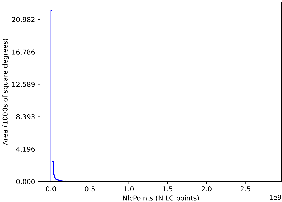
internal_u_expt60_nscale1.0v3.4_10yrs : NlcPoints
