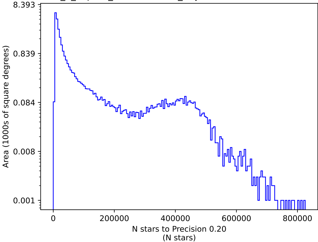
internal_u_expt60_nscale1.0v3.4_10yrs i: N stars to Precision 0.20
