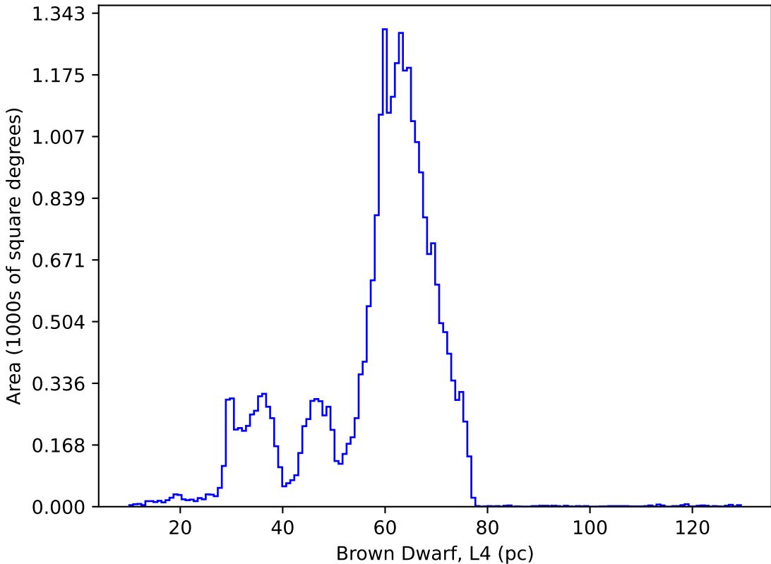
internal_u_expt60_nscale1.0v3.4_10yrs : Brown Dwarf, L4
