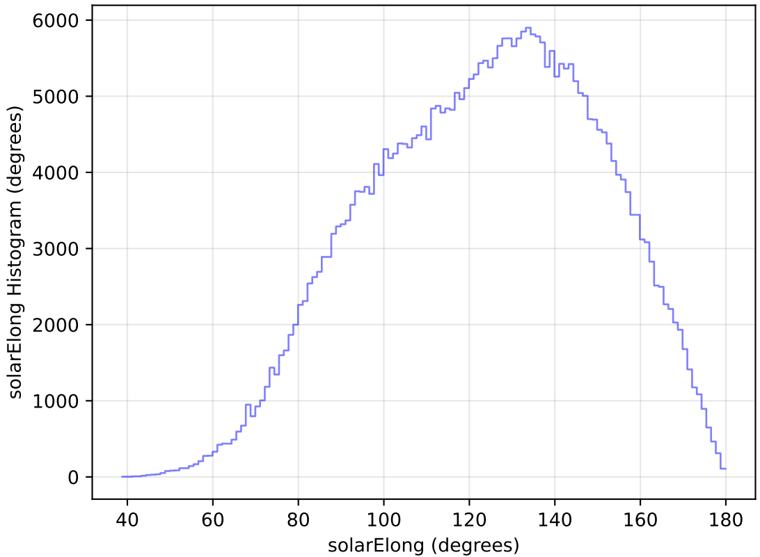
internal_u_expt60_nscale1.0v3.4_10yrs WFD y band: solarElong Histogram
