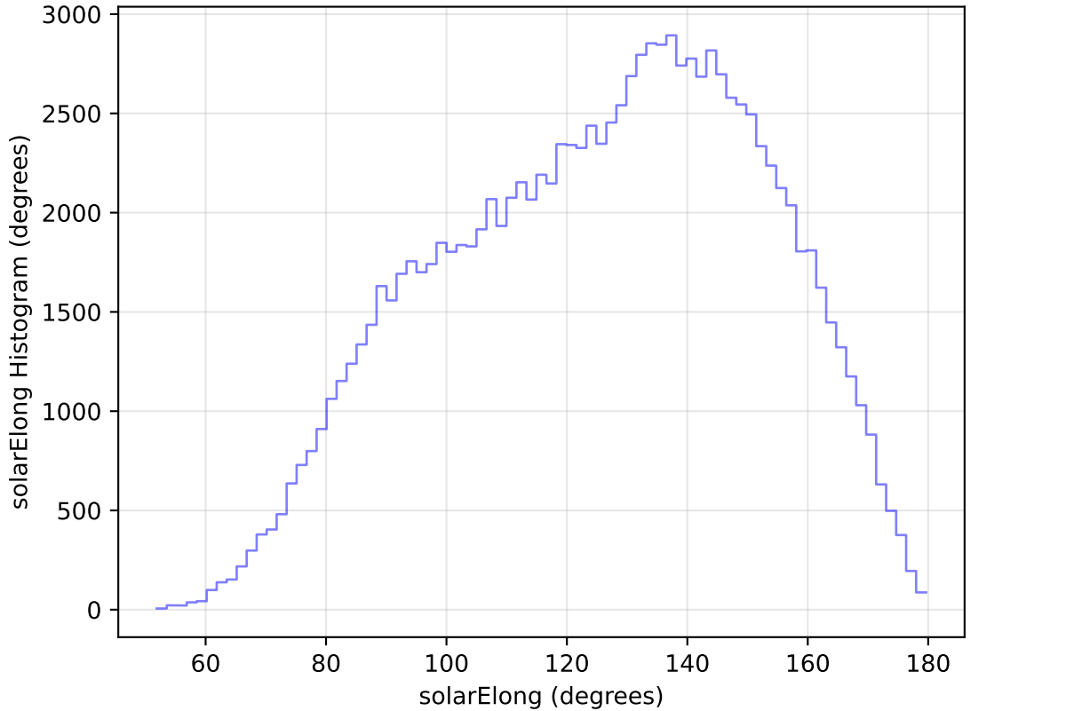
internal_u_expt60_nscale1.0v3.4_10yrs WFD u band: solarElong Histogram
