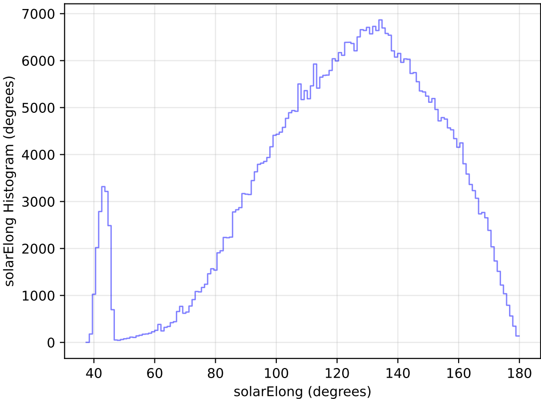
internal_u_expt60_nscale1.0v3.4_10yrs WFD r band: solarElong Histogram
