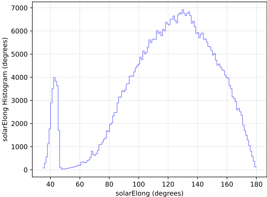
internal_u_expt60_nscale1.0v3.4_10yrs WFD i band: solarElong Histogram
