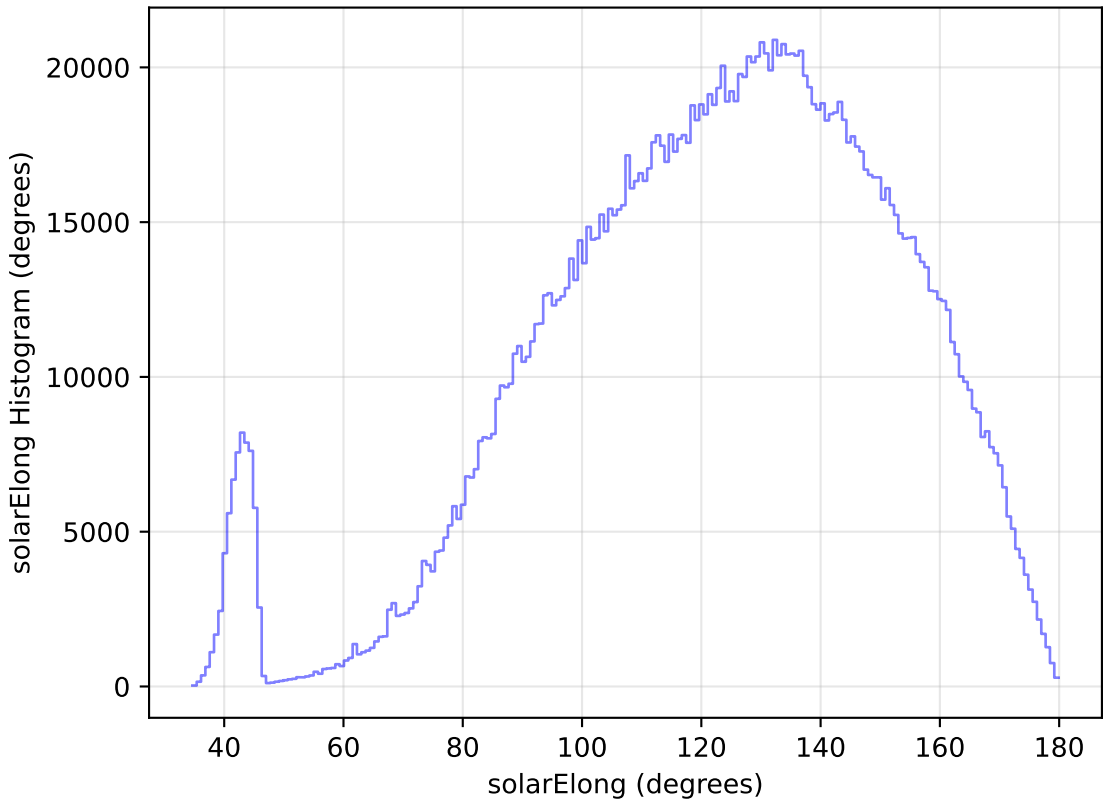
internal_u_expt60_nscale1.0v3.4_10yrs WFD all bands: solarElong Histogram
