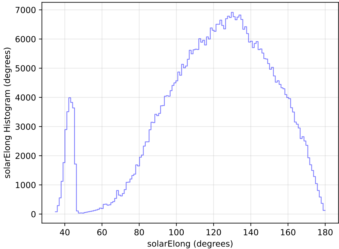
internal_u_expt60_nscale1.0v3.4_10yrs All sky i band: solarElong Histogram
