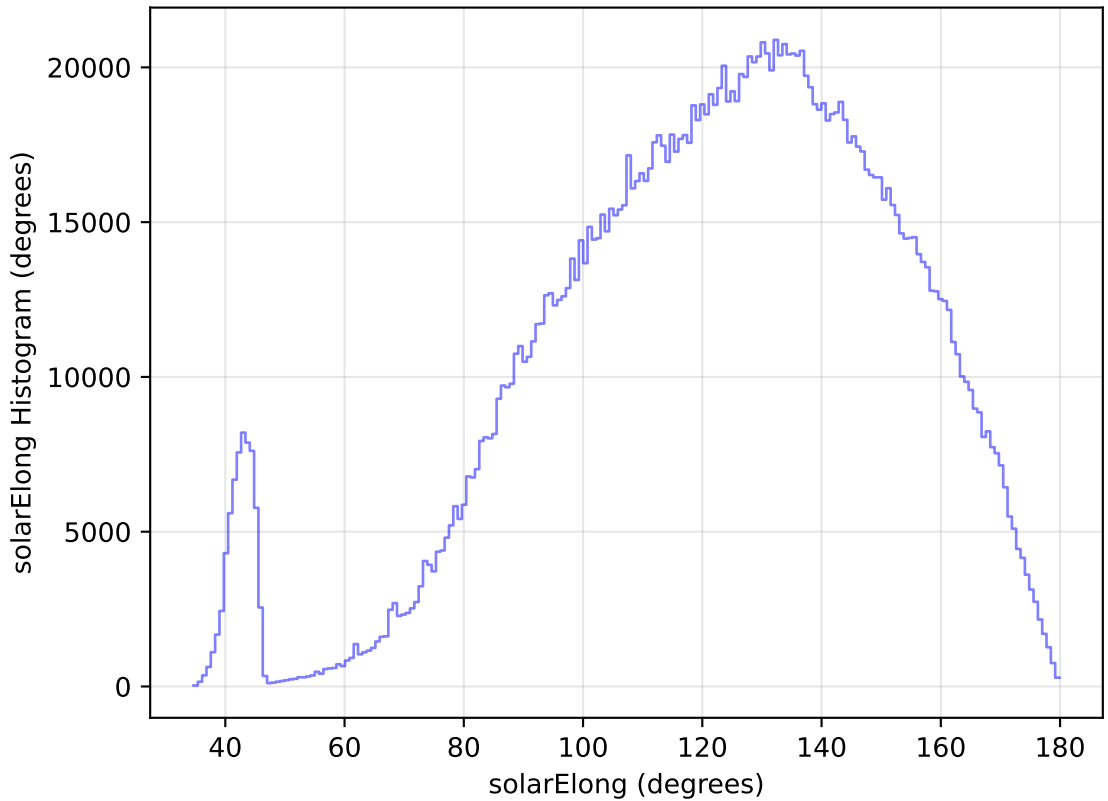
internal_u_expt60_nscale1.0v3.4_10yrs All sky all bands: solarElong Histogram
