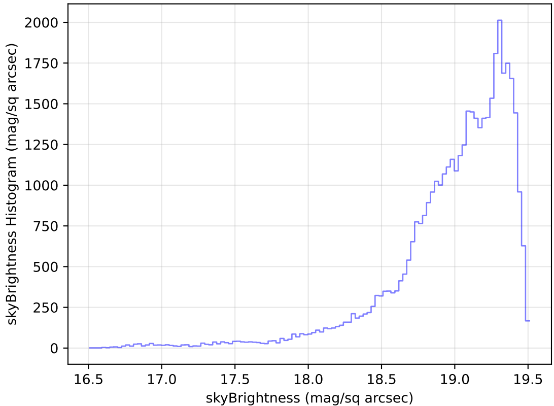
internal_u_expt60_nscale1.0v3.4_10yrs Yr 1 z band: skyBrightness Histogram
