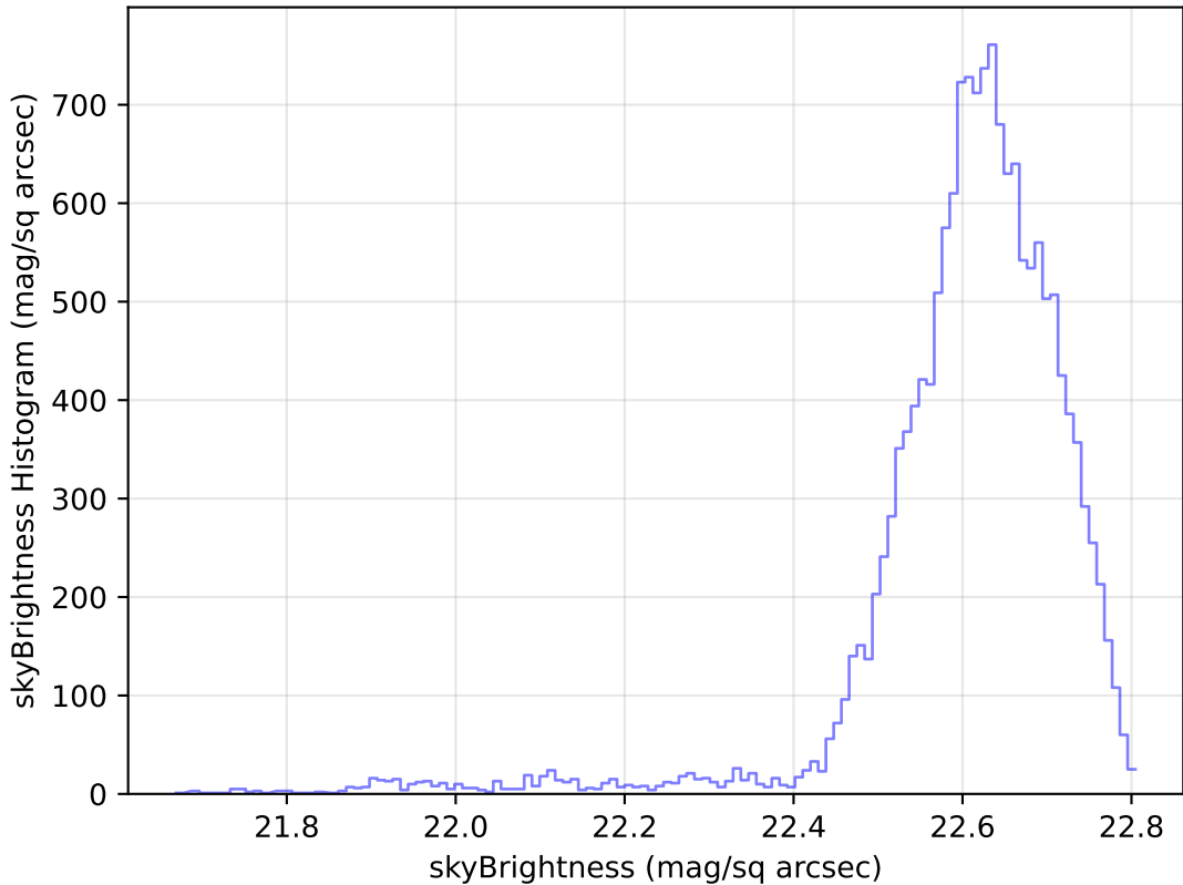
internal_u_expt60_nscale1.0v3.4_10yrs Yr 1 u band: skyBrightness Histogram
