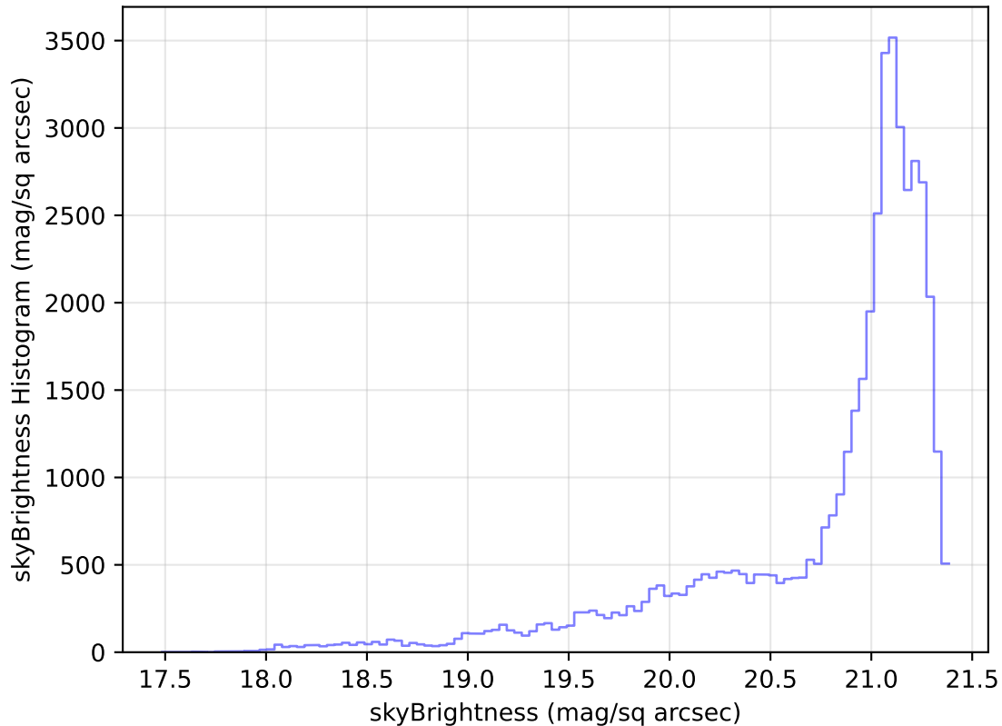
internal_u_expt60_nscale1.0v3.4_10yrs Yr 1 r band: skyBrightness Histogram
