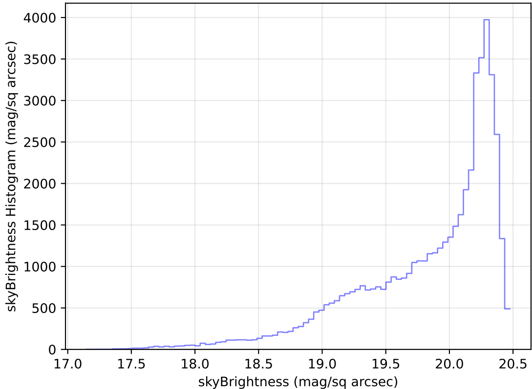
internal_u_expt60_nscale1.0v3.4_10yrs Yr 1 i band: skyBrightness Histogram
