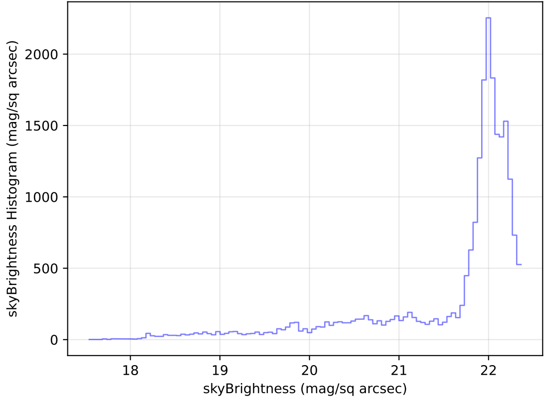
internal_u_expt60_nscale1.0v3.4_10yrs Yr 1 g band: skyBrightness Histogram
