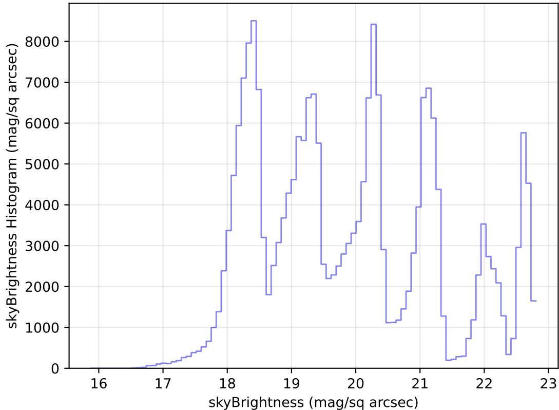
internal_u_expt60_nscale1.0v3.4_10yrs Yr 1 all bands: skyBrightness Histogram
