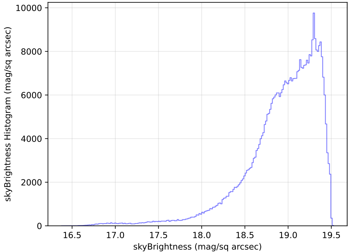
internal_u_expt60_nscale1.0v3.4_10yrs WFD z band: skyBrightness Histogram
