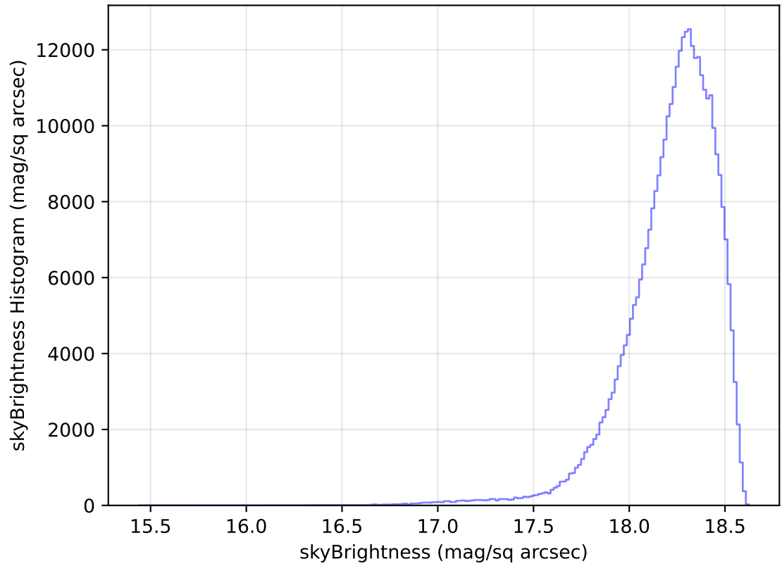
internal_u_expt60_nscale1.0v3.4_10yrs WFD y band: skyBrightness Histogram
