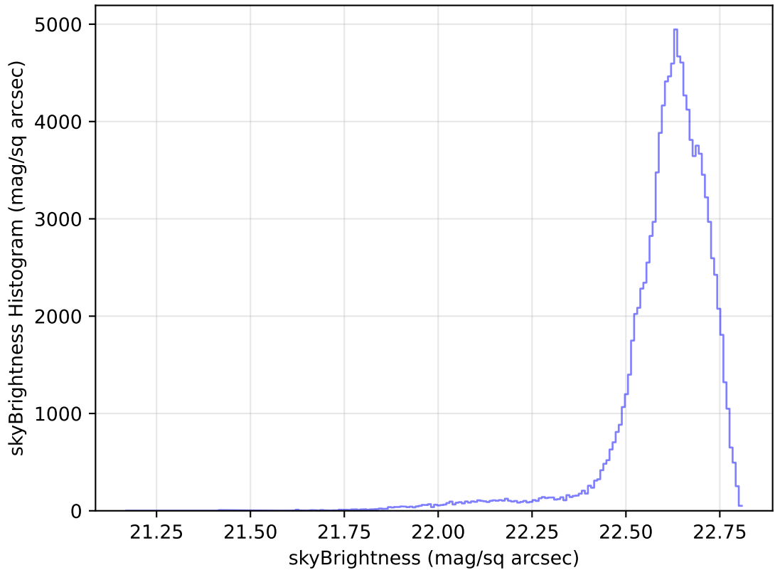
internal_u_expt60_nscale1.0v3.4_10yrs WFD u band: skyBrightness Histogram
