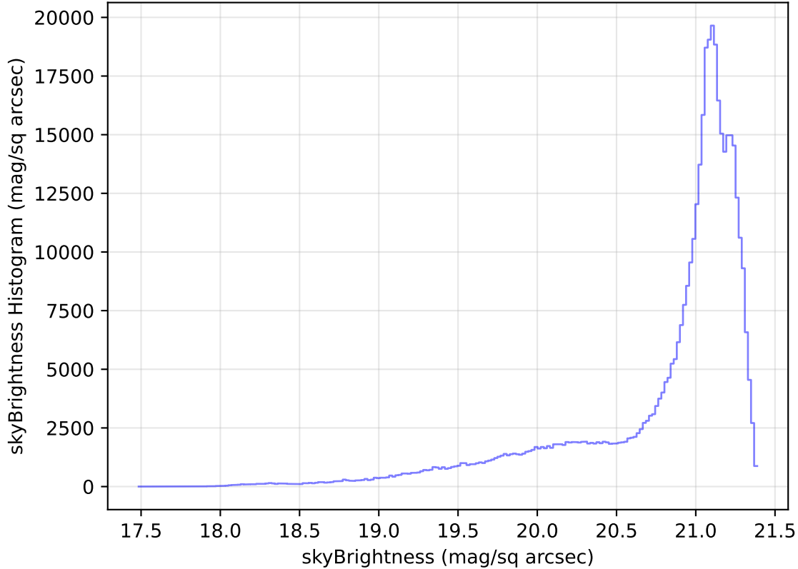
internal_u_expt60_nscale1.0v3.4_10yrs WFD r band: skyBrightness Histogram
