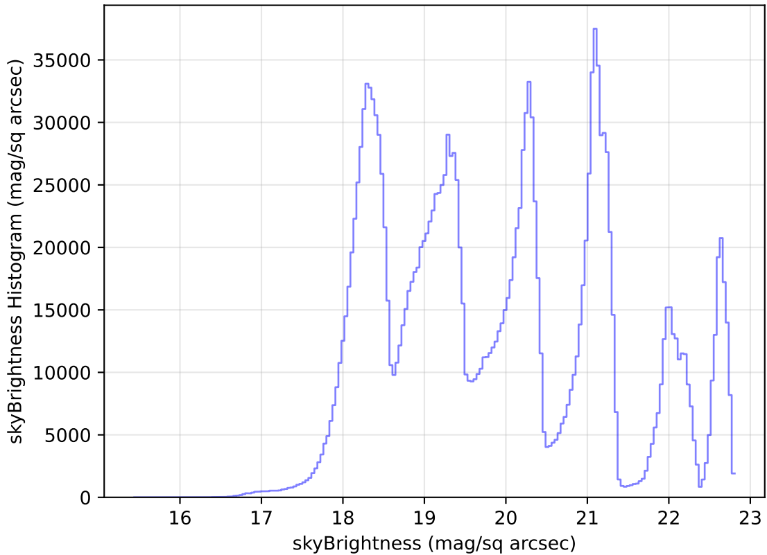
internal_u_expt60_nscale1.0v3.4_10yrs WFD all bands: skyBrightness Histogram
