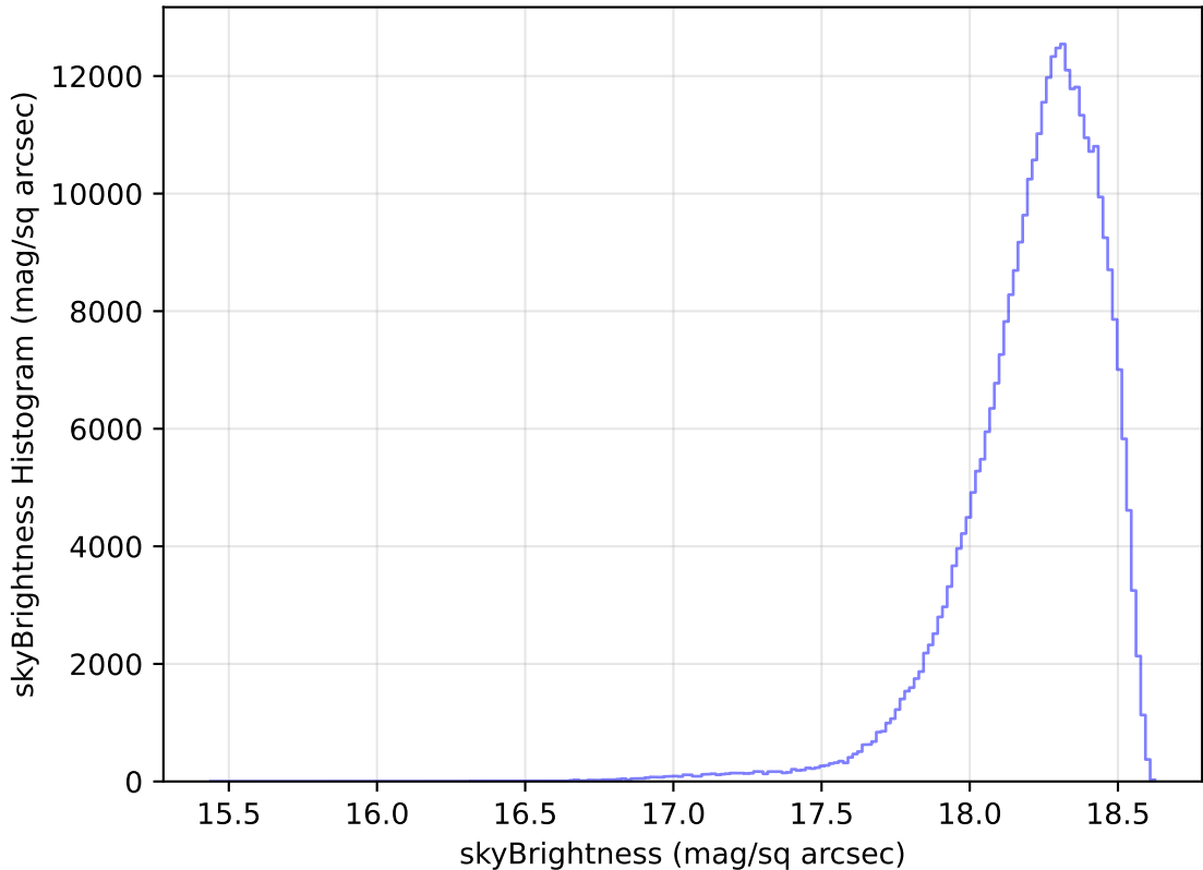
internal_u_expt60_nscale1.0v3.4_10yrs All sky y band: skyBrightness Histogram
