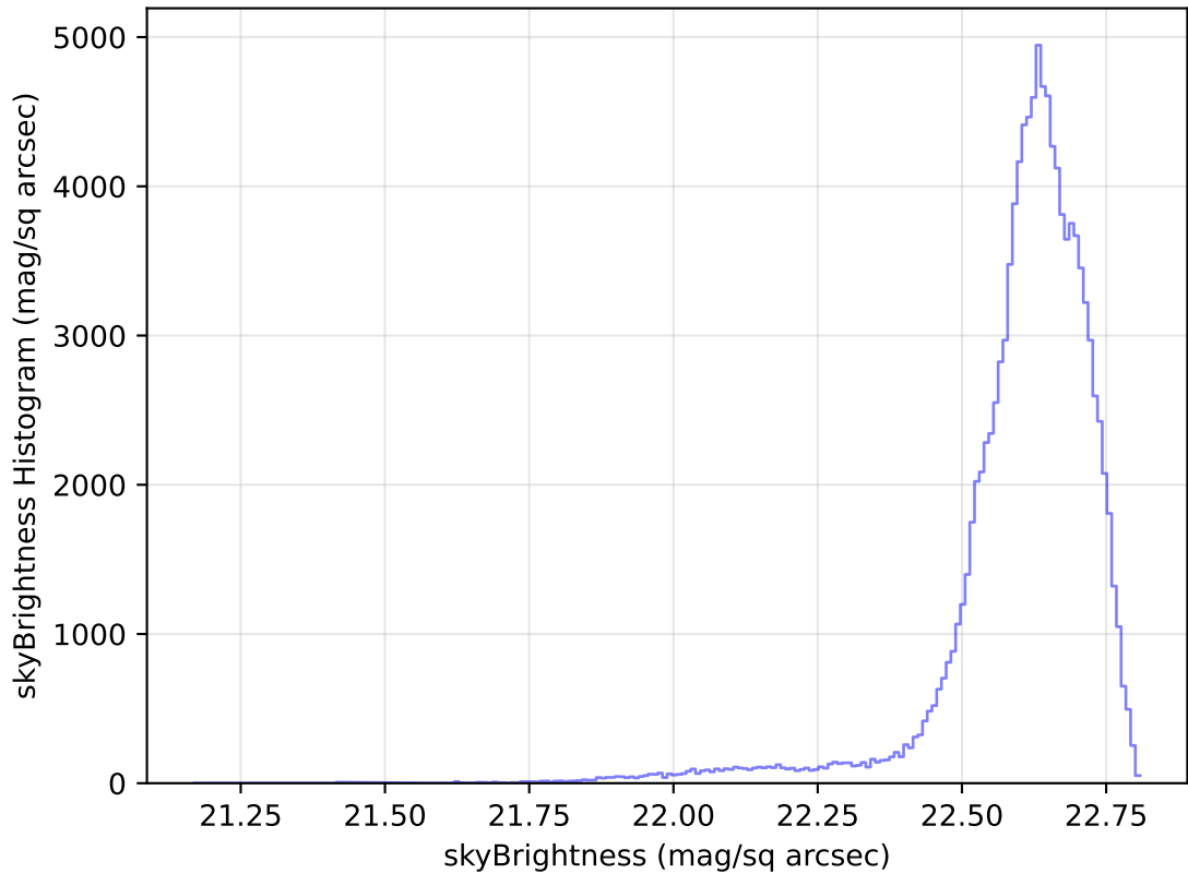
internal_u_expt60_nscale1.0v3.4_10yrs All sky u band: skyBrightness Histogram
