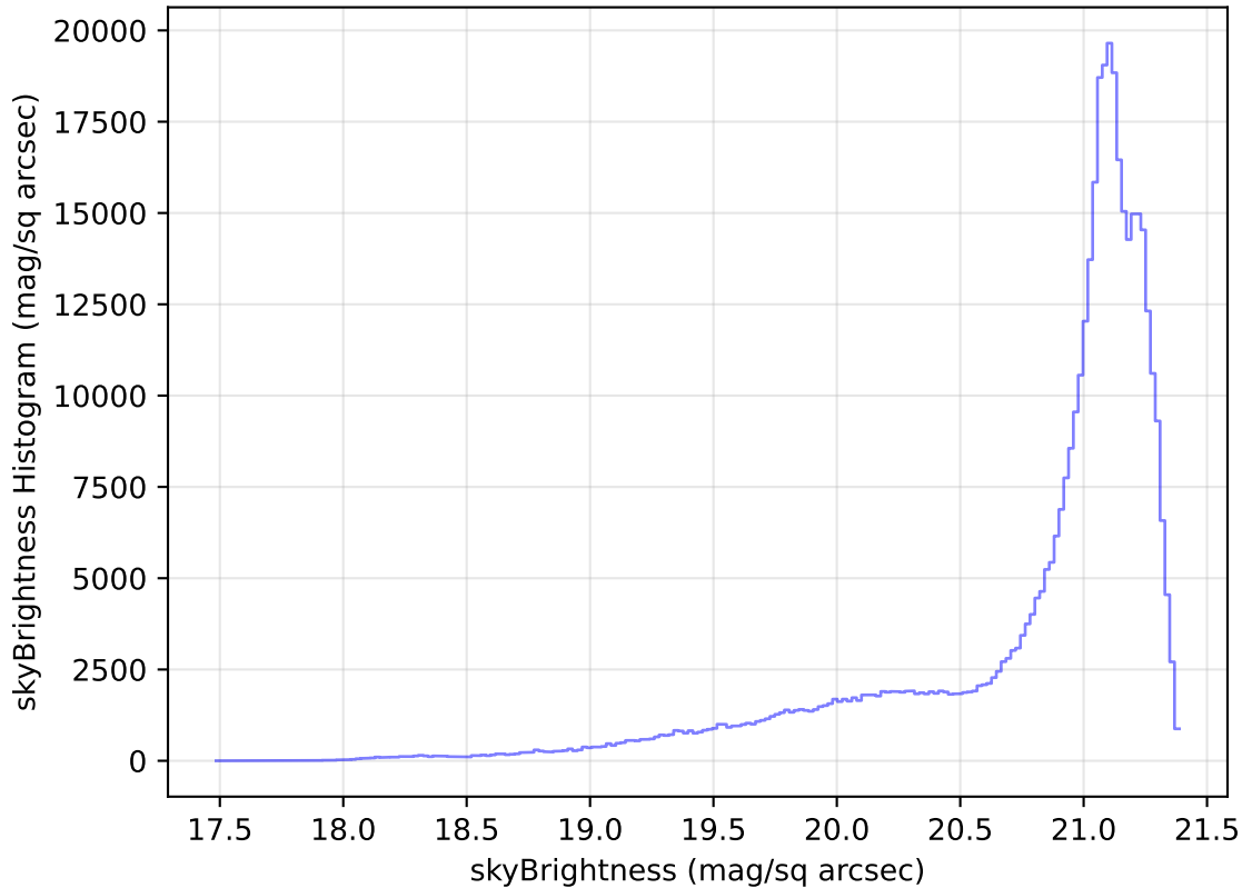
internal_u_expt60_nscale1.0v3.4_10yrs All sky r band: skyBrightness Histogram
