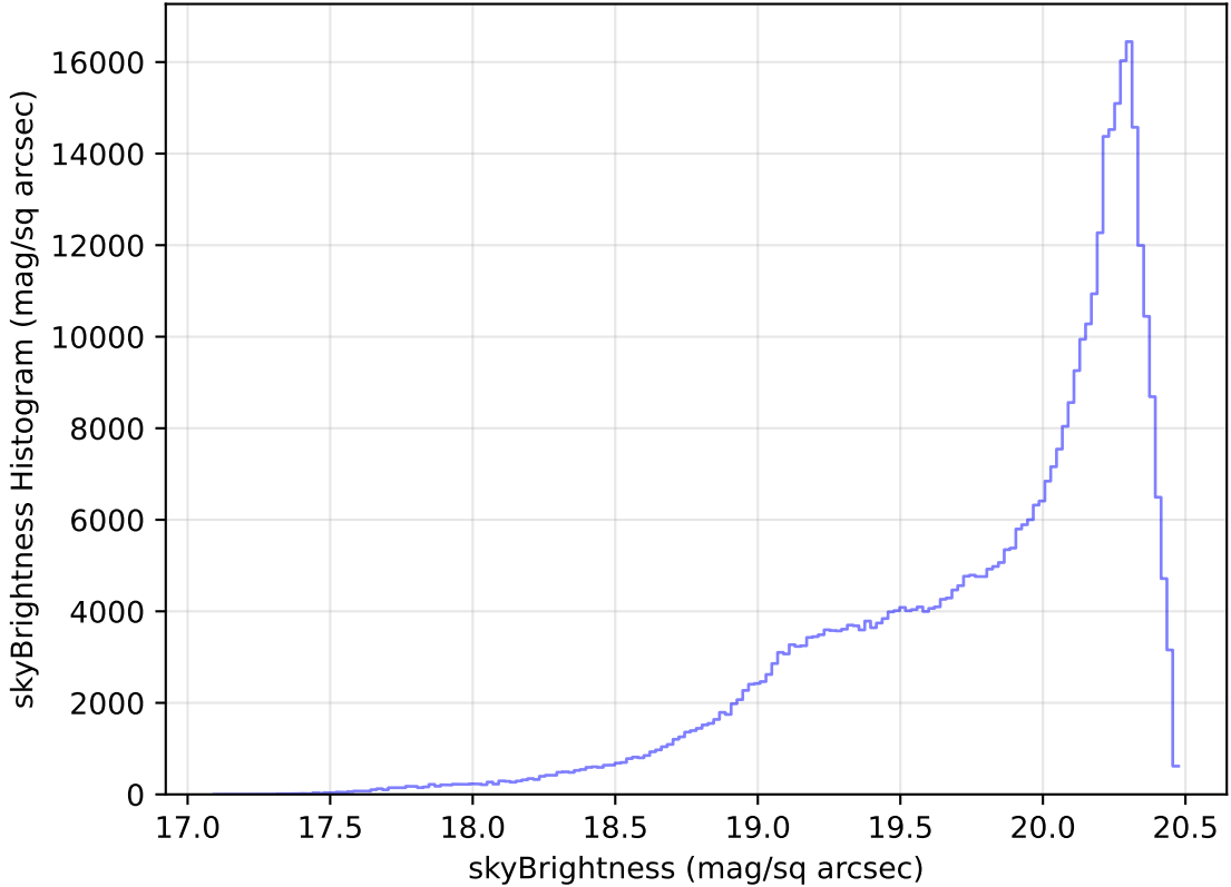
internal_u_expt60_nscale1.0v3.4_10yrs All sky i band: skyBrightness Histogram
