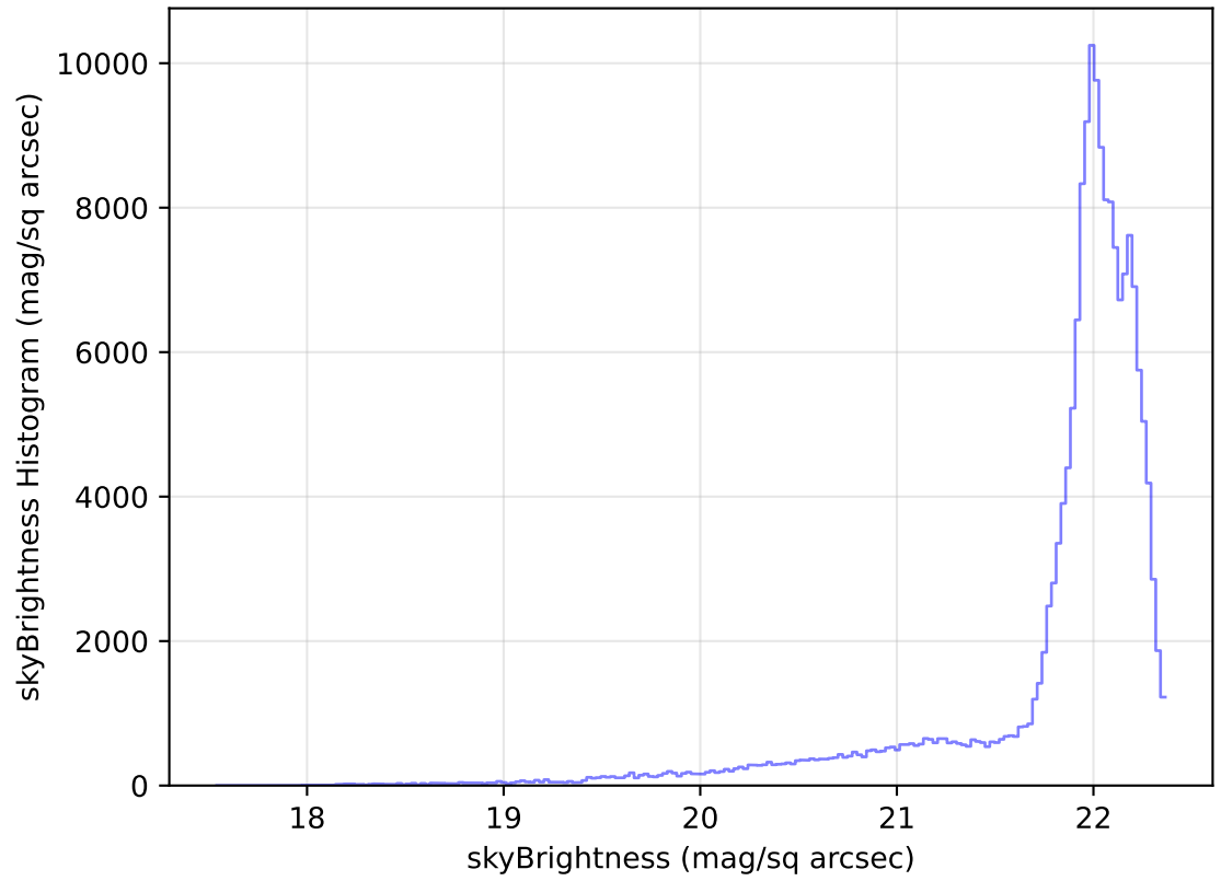
internal_u_expt60_nscale1.0v3.4_10yrs All sky g band: skyBrightness Histogram
