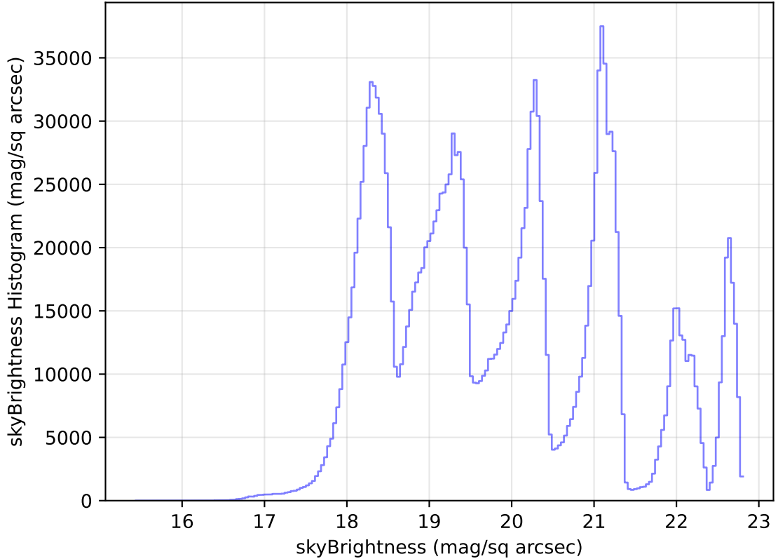
internal_u_expt60_nscale1.0v3.4_10yrs All sky all bands: skyBrightness Histogram
