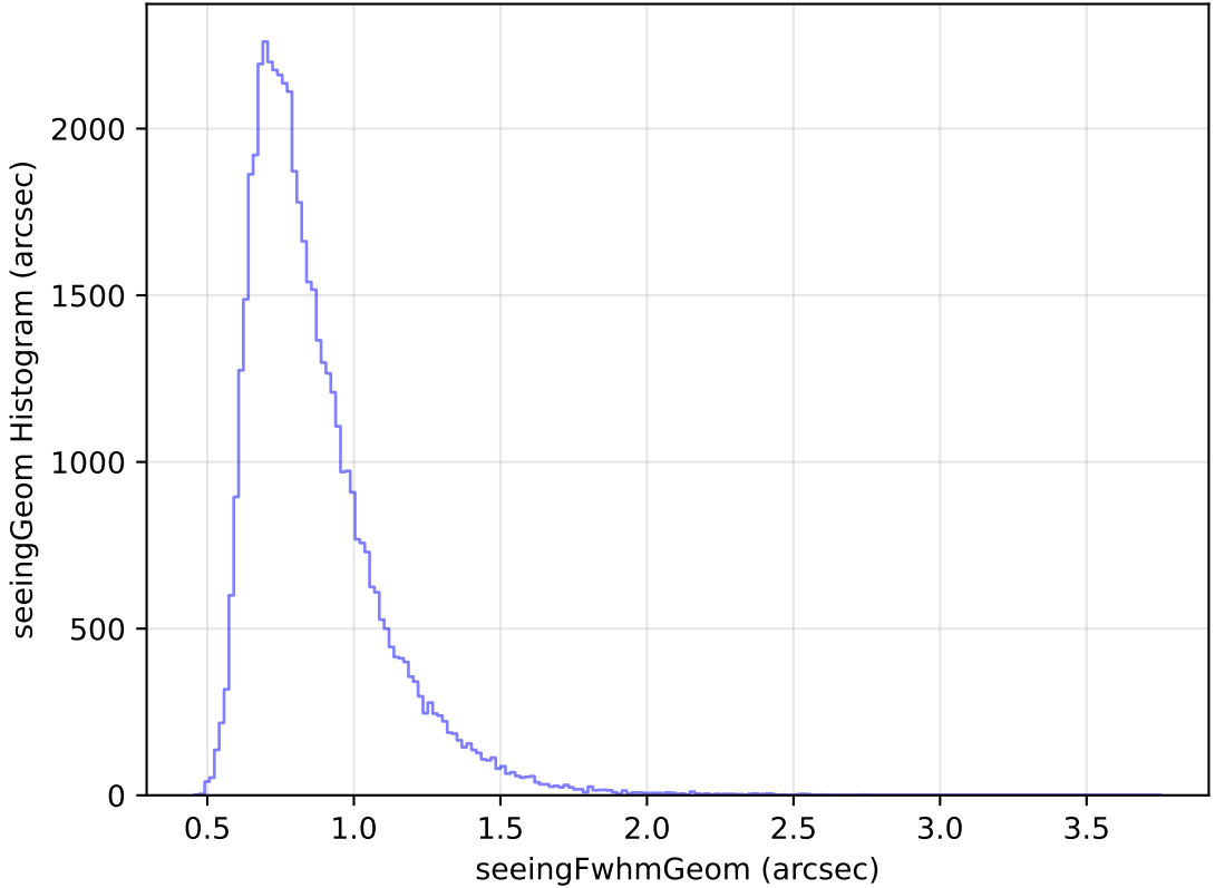
internal_u_expt60_nscale1.0v3.4_10yrs Yr 1 i band: seeingGeom Histogram
