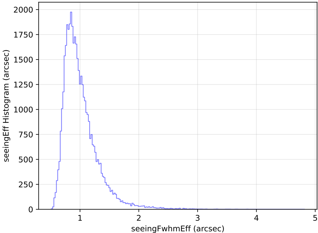
internal_u_expt60_nscale1.0v3.4_10yrs Yr 1 z band: seeingEff Histogram
