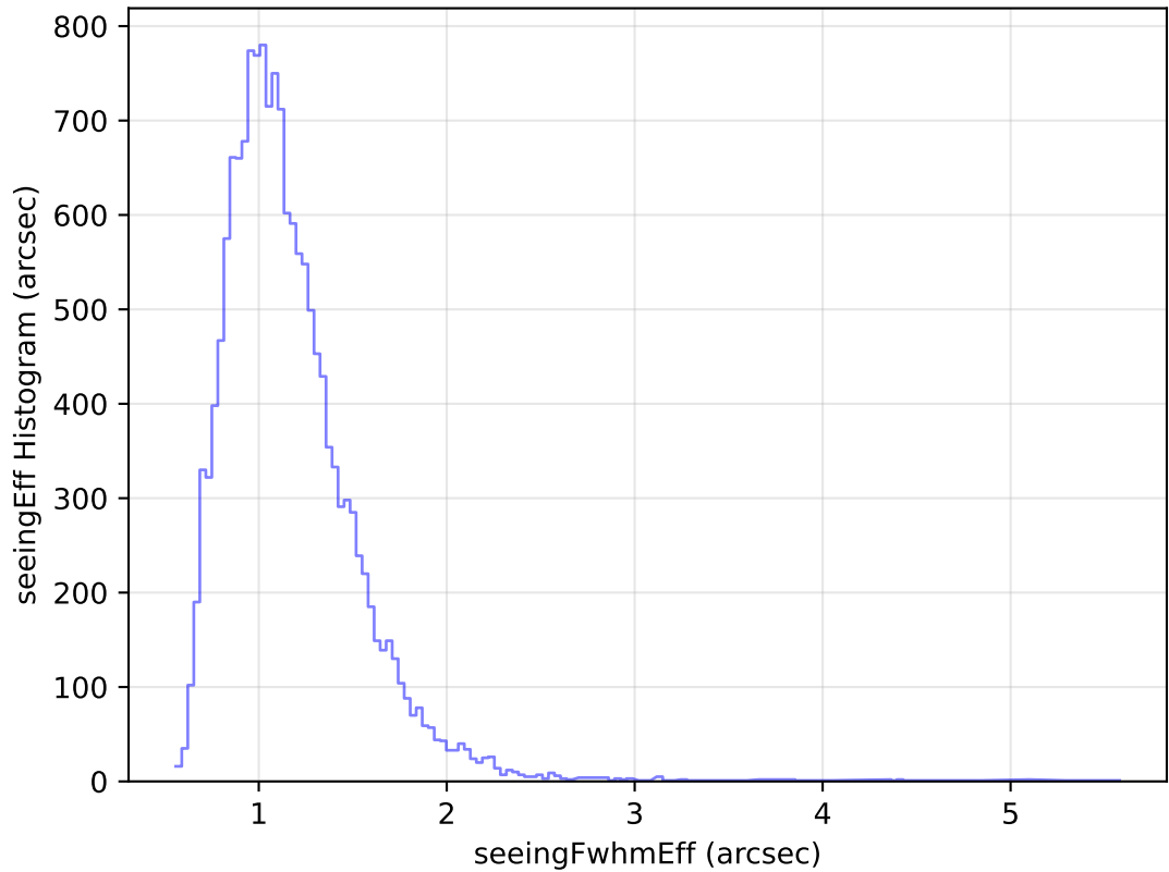
internal_u_expt60_nscale1.0v3.4_10yrs Yr 1 u band: seeingEff Histogram
