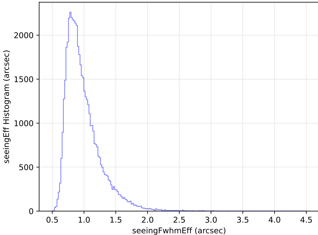
internal_u_expt60_nscale1.0v3.4_10yrs Yr 1 i band: seeingEff Histogram
