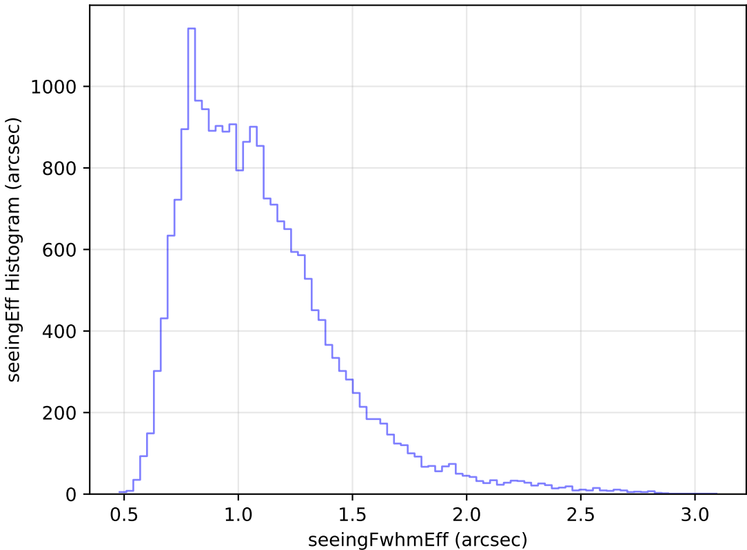
internal_u_expt60_nscale1.0v3.4_10yrs Yr 1 g band: seeingEff Histogram
