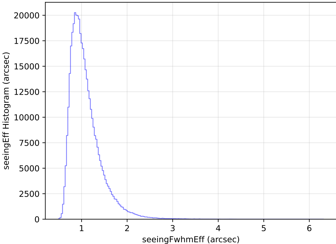
internal_u_expt60_nscale1.0v3.4_10yrs WFD z band: seeingEff Histogram
