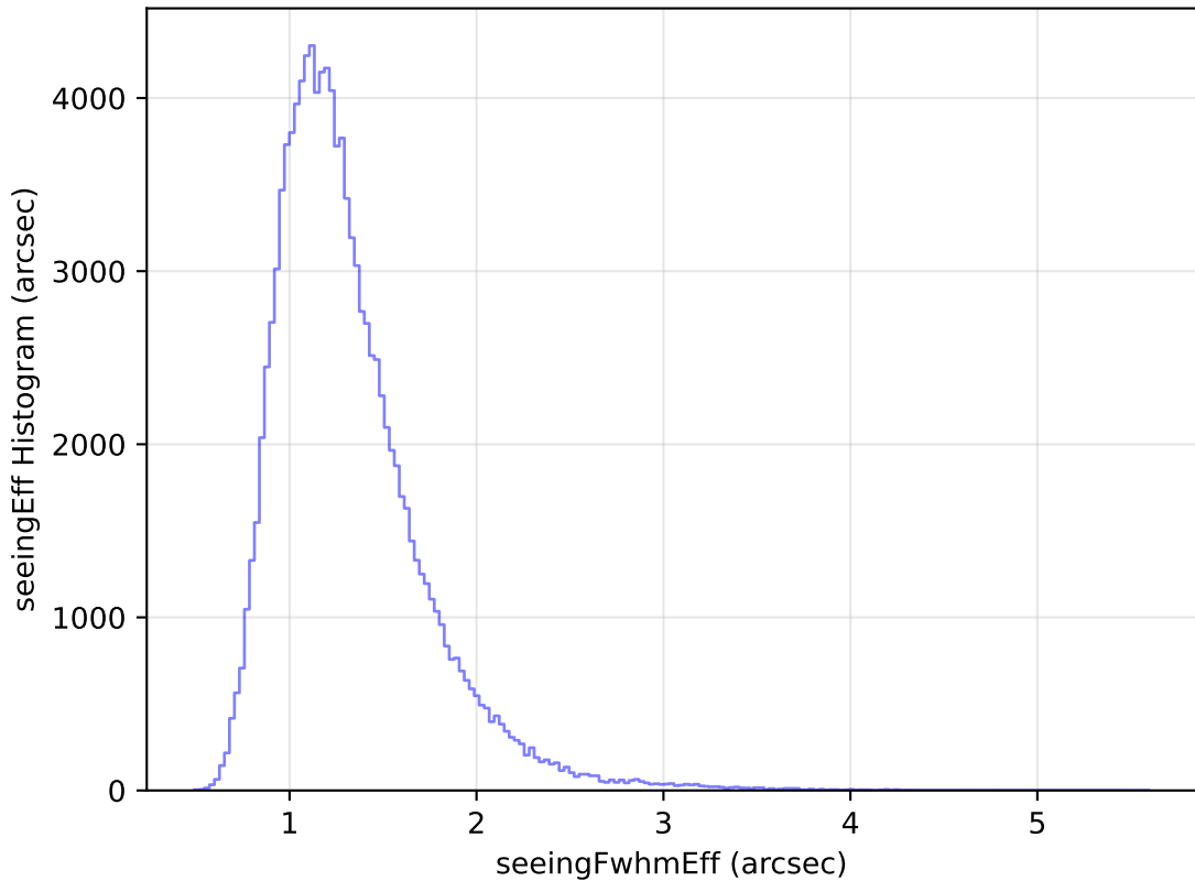
internal_u_expt60_nscale1.0v3.4_10yrs WFD u band: seeingEff Histogram
